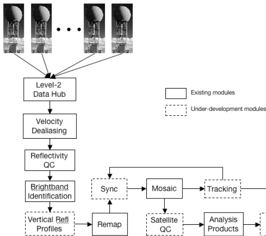
Fig. 1. An overview flowchart of the NMQ 3D high-resolution radar mosaic system.
